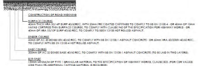
THE STREET ROAD WIDENING CONSTRUCTION DETAIL Not to Scale
