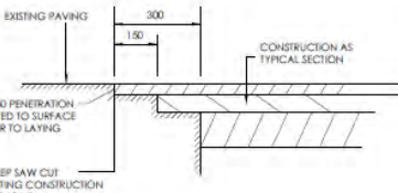
TYPICAL DETAIL TIE-IN BETWEEN NEW & EXISTING BITUMINOUS CONSTRUCTION SCALE 1:10
